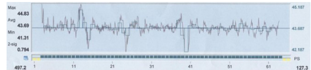
Figure 2. Dry weight profile before service
