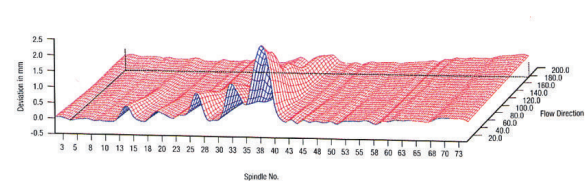
Figure 4. Example of a damaged headbox apron
